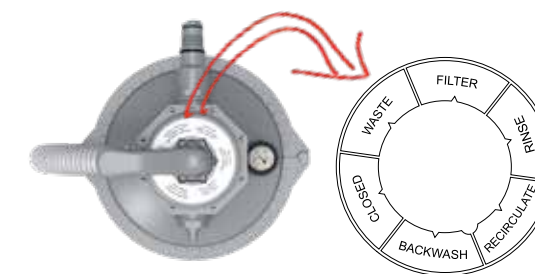
6-position valve
