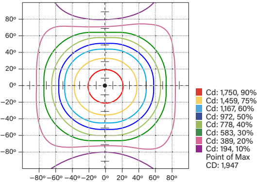
ISOCANDELA PLOT
