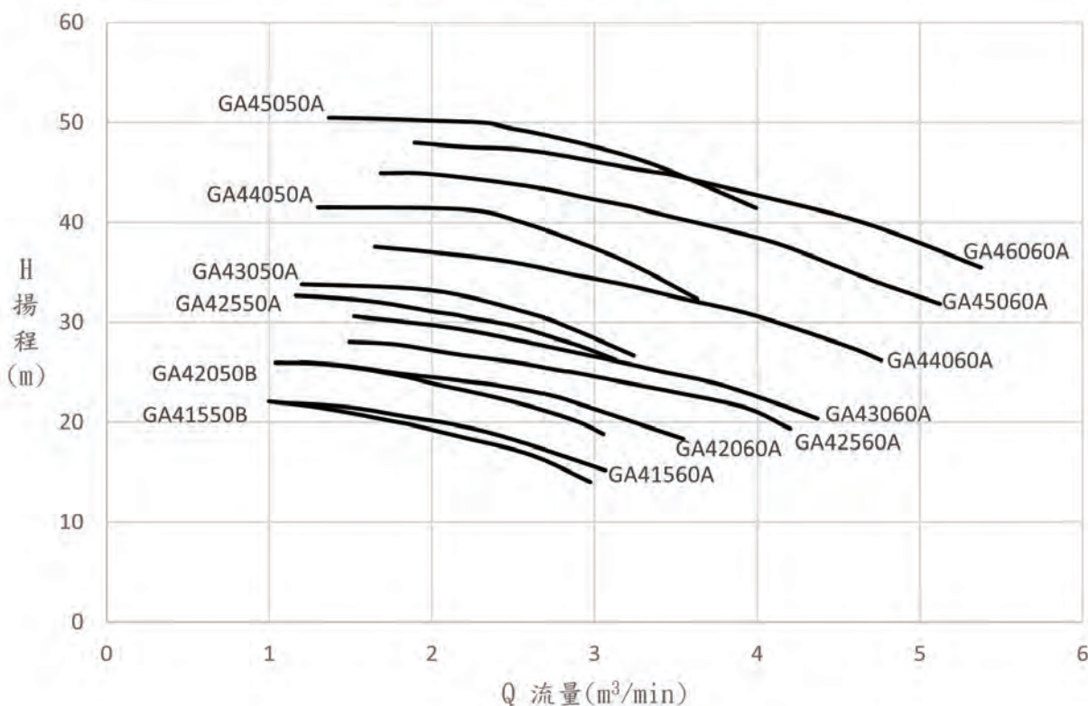
4P流量-揚程性能曲線圖(2/3)
