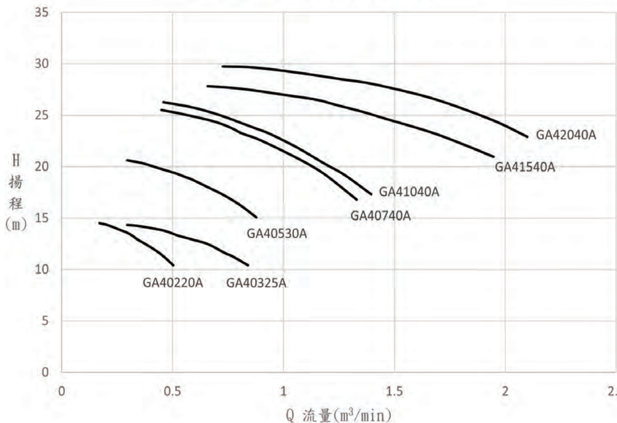
4P流量-揚程性能曲線圖(1/3)
