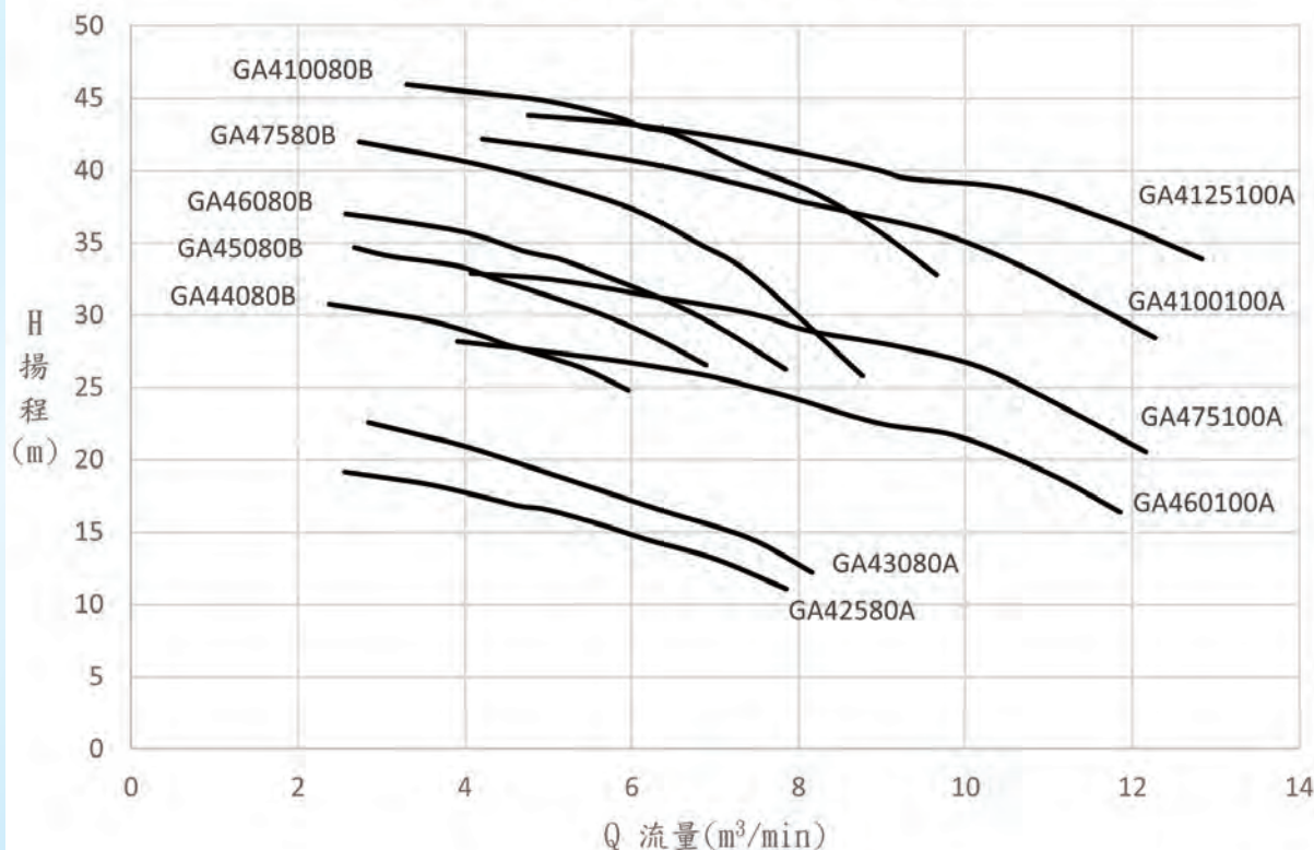
4P流量-揚程性能曲線圖(3/3)
