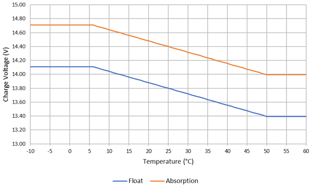
Charge Voltage - Temperature Compensation
