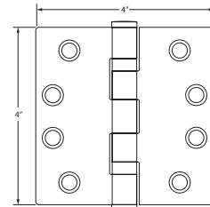
4" Hinge
