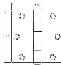
3-1/2" Hinge
