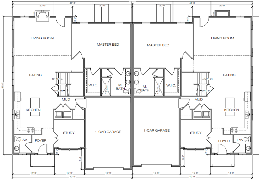
FIRST FLOOR PLAN 9' CEILING HEIGHT 1,485 Sq.Ft.
