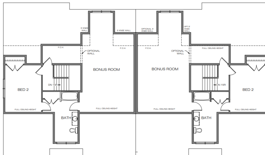
SECOND FLOOR PLAN 8' CEILING HEIGHT 974 Sq.Ft.
