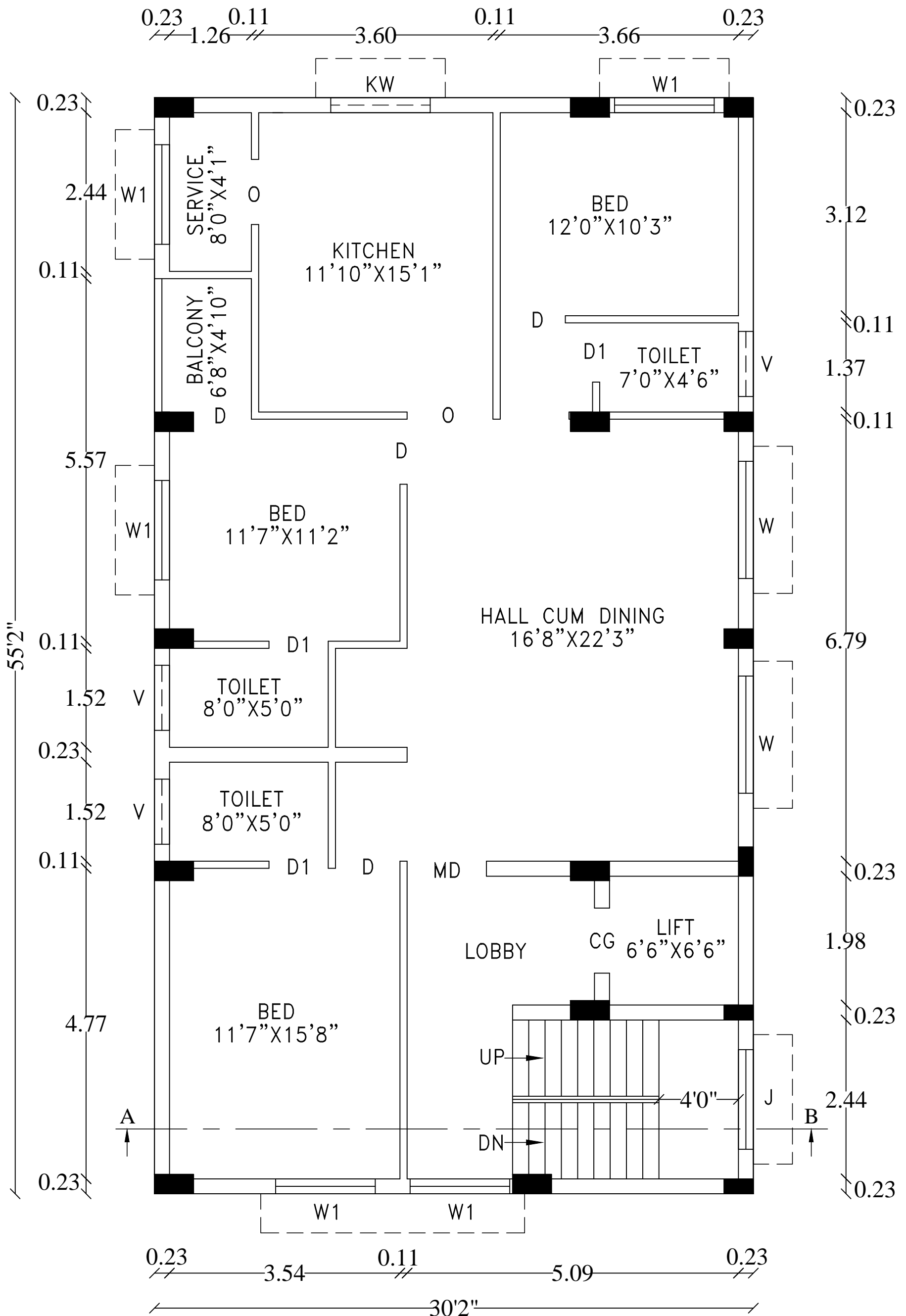
TYPICAL FLOOR PLAN THILLAI NAGAR 10TH CROSS PLAN
