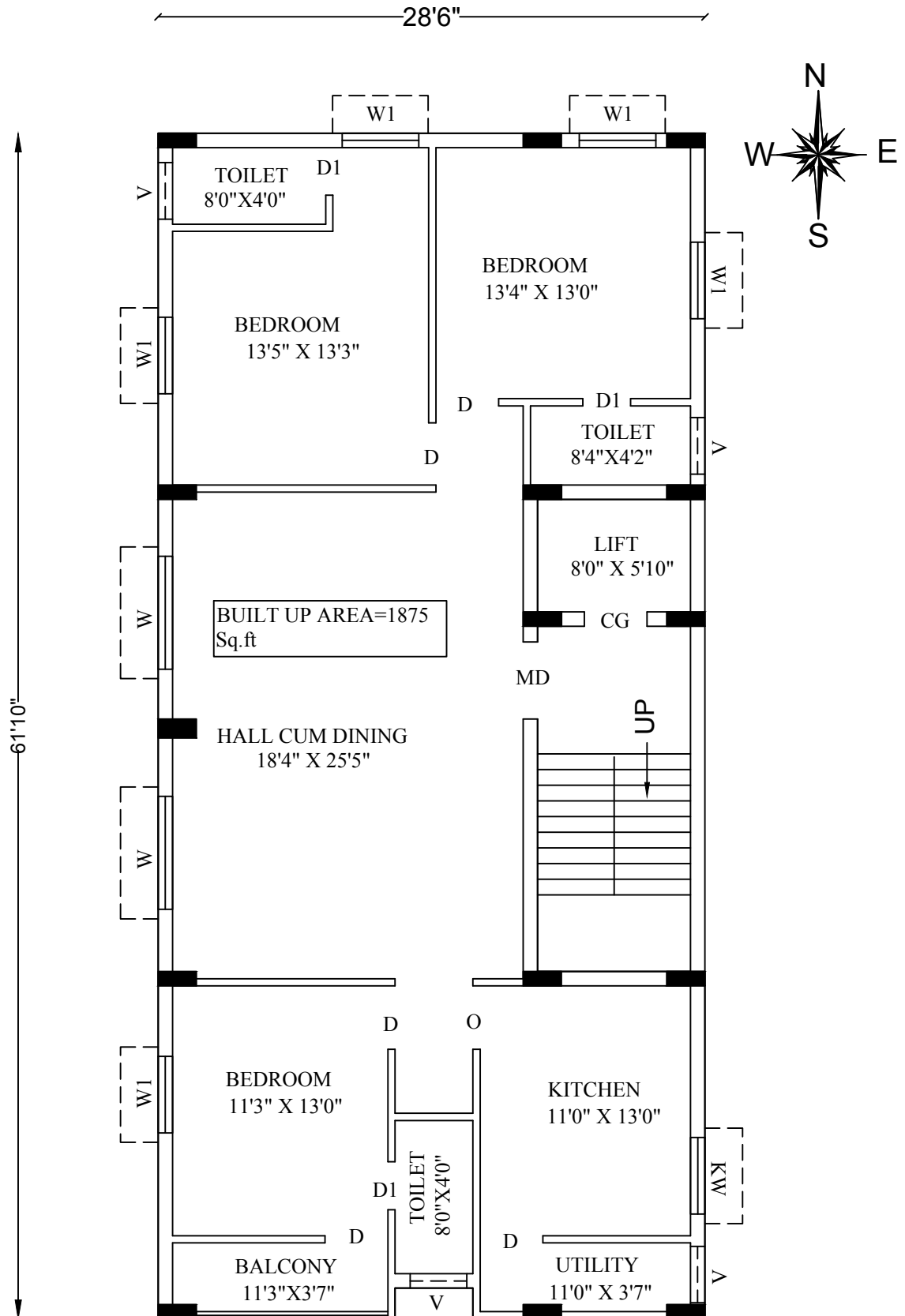
TYPICAL FLOOR PLAN KAMARAJAR ST, KK NAGAR
