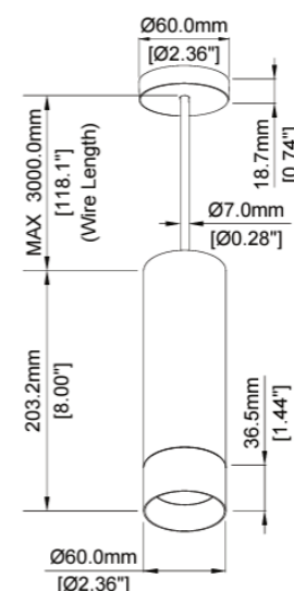
Dimension Drawings
