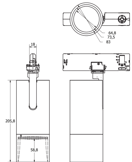
Dimension Drawings
