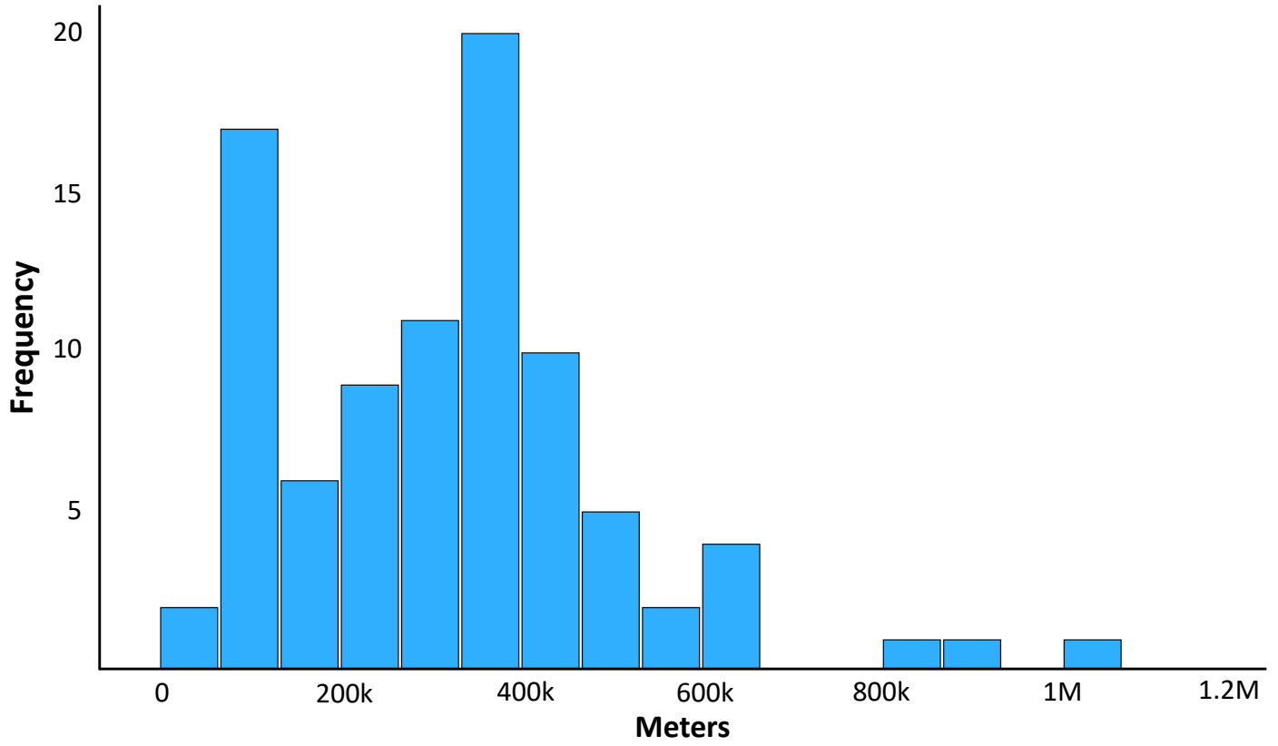
Schwarzschild Diameter (Linear)
