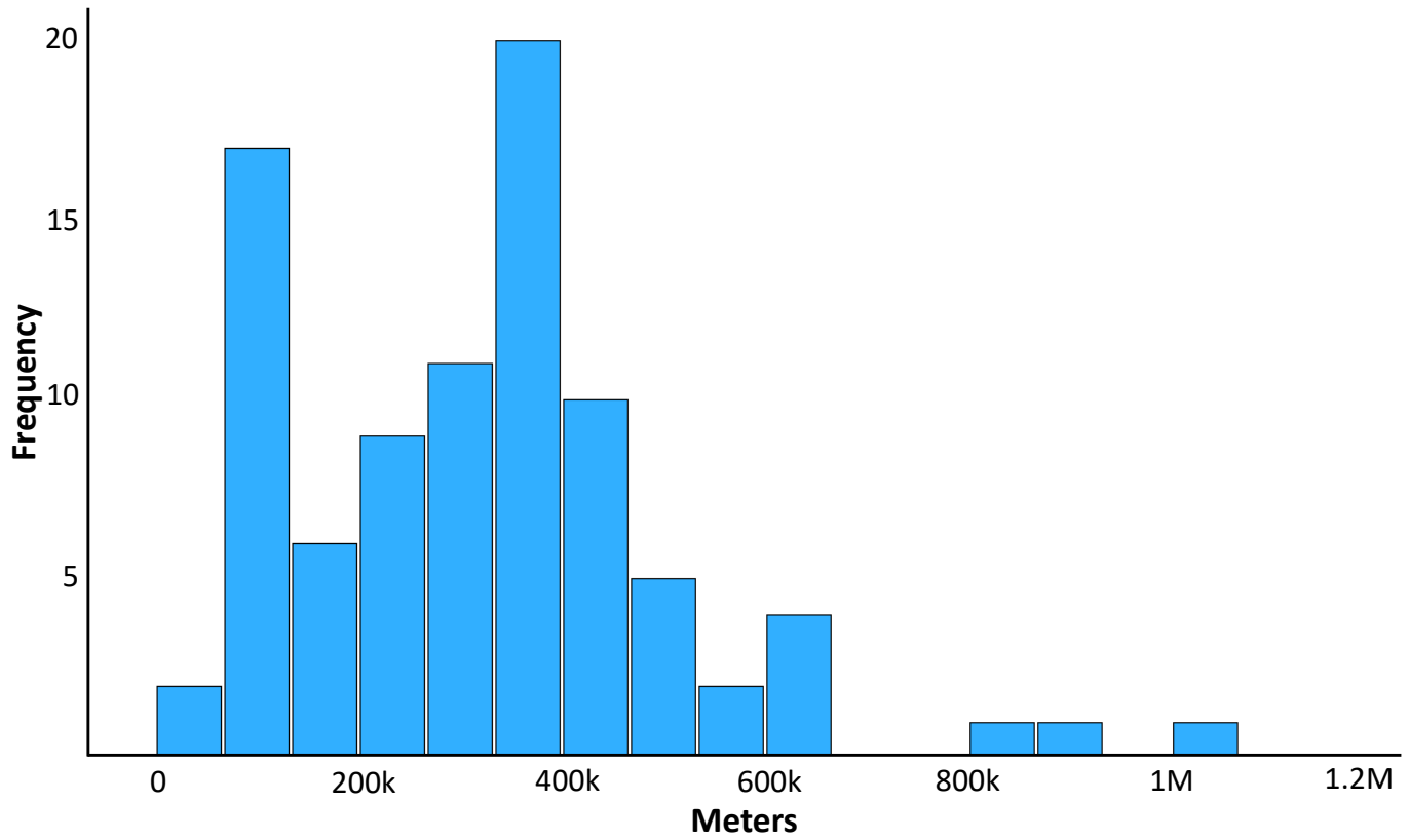
Schwarzschild Diameter (Linear)
