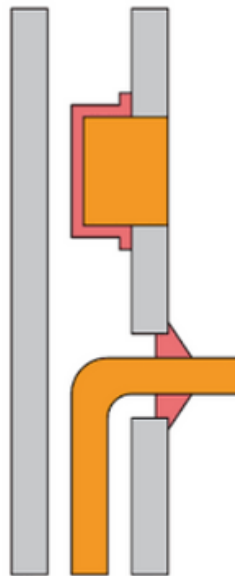
Membrane Penetration
