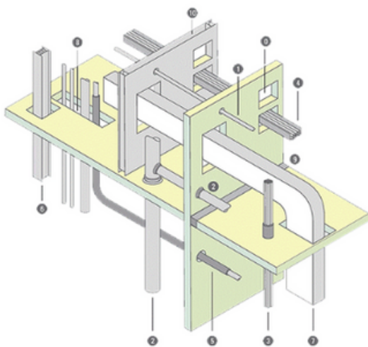
MEP PENETRATIONS
