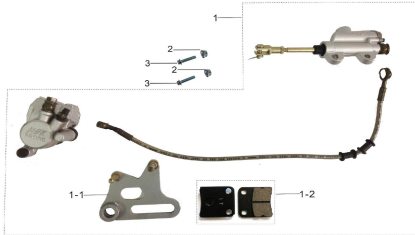
REAR BRAKE ASSY.
