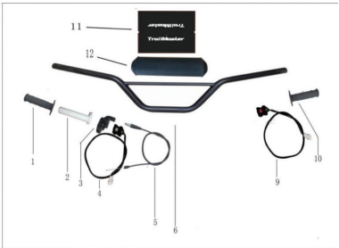
STEERING ASSY.
