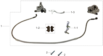
FRONT BRAKE ASSY.
