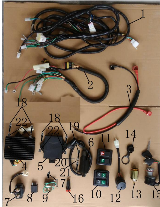
FIG. 37 ELECTRICAL PARTS 1
