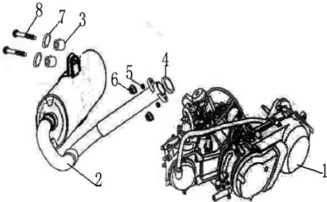
FIG. 29 ENGINE & EXHAUST
