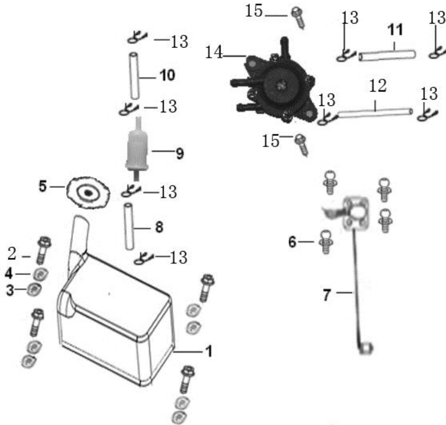
FIG. 36 FUEL TANK
