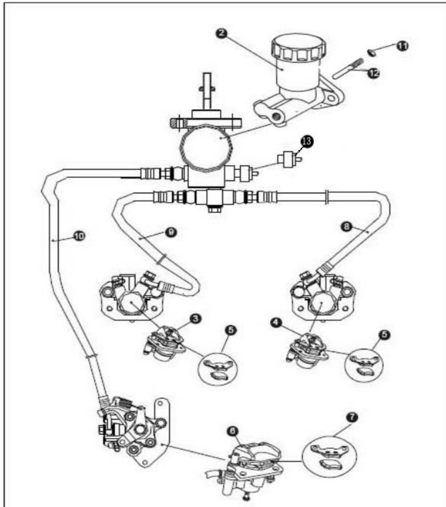
FIG. 34 BRAKE ASSY. 1
