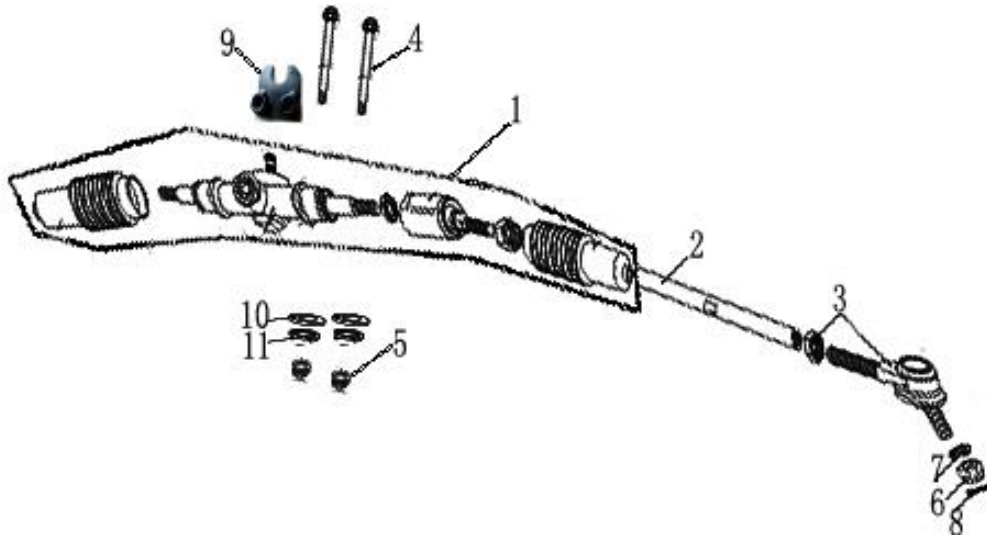
FIG. 26 STEERING GEAR
