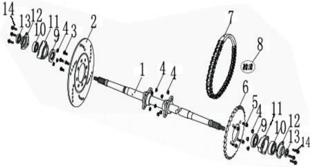
FIG. 33 REAR AXLE
