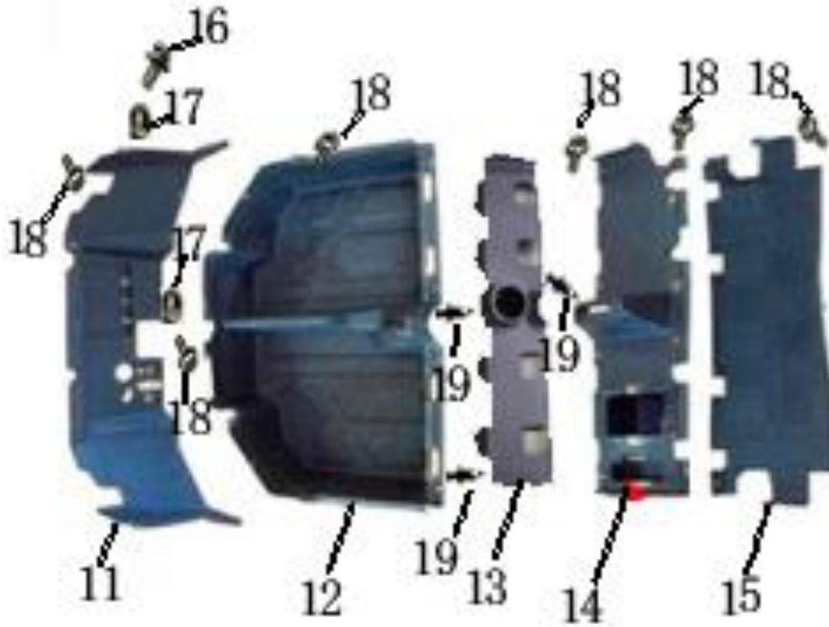
FIG. 40 PLASTIC PARTS 2
