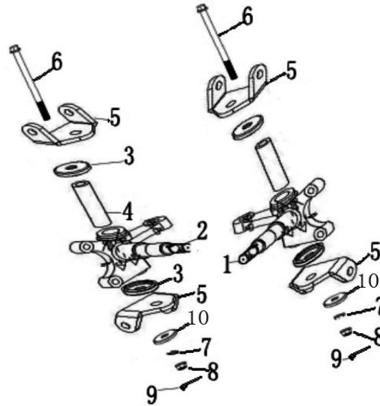
FIG 21 FRONT SPINDLE
