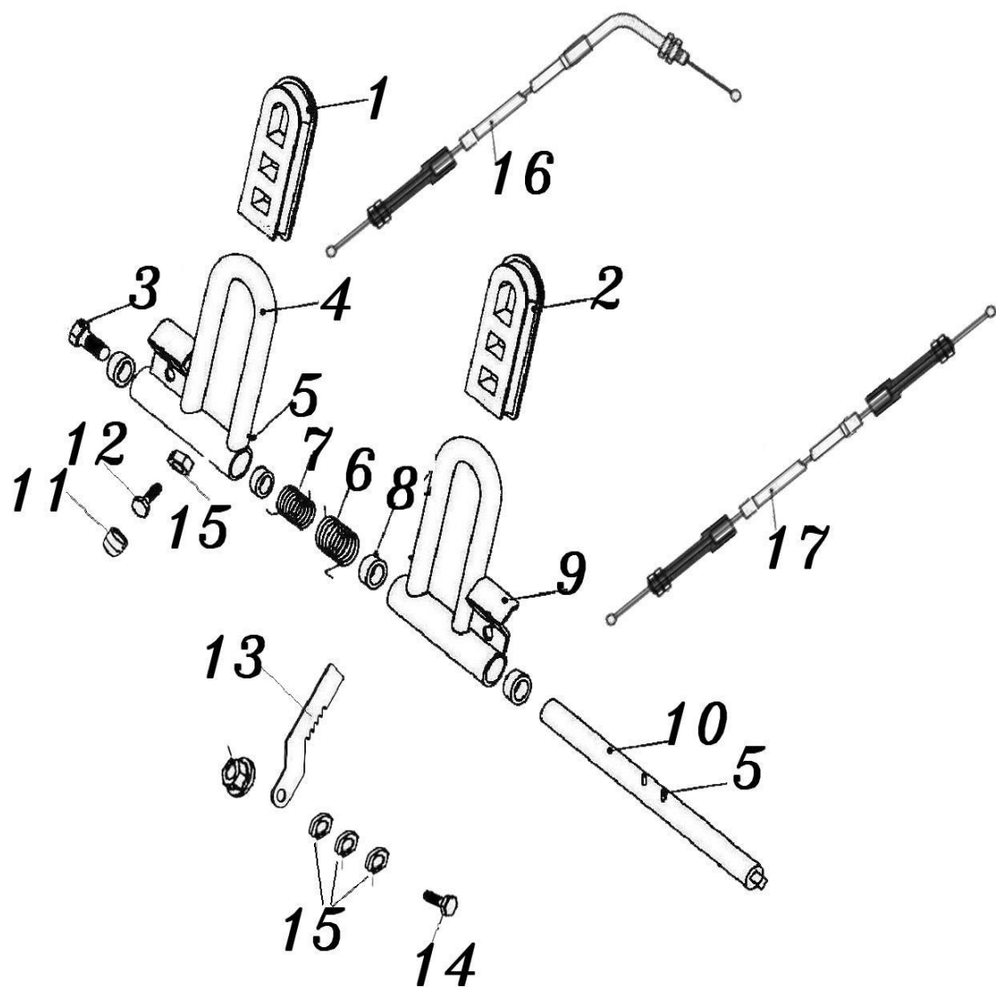
FIG:4 左右转向摇臂 SPINDLE AND STRUT SUPPORT
