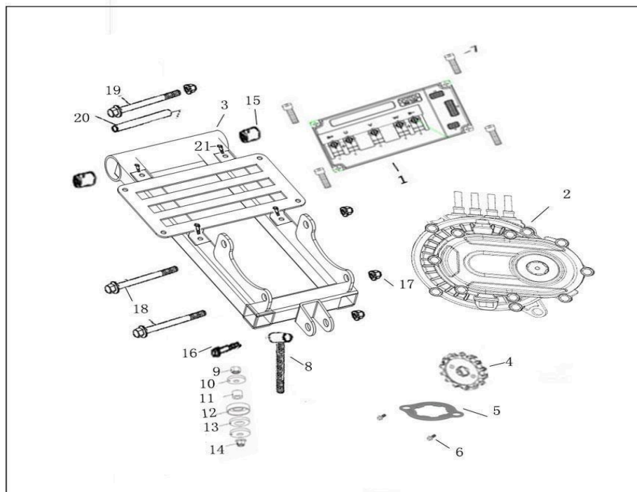
Fig 6: ELECTRIC MOTOR/CONTROLLER ASSY
