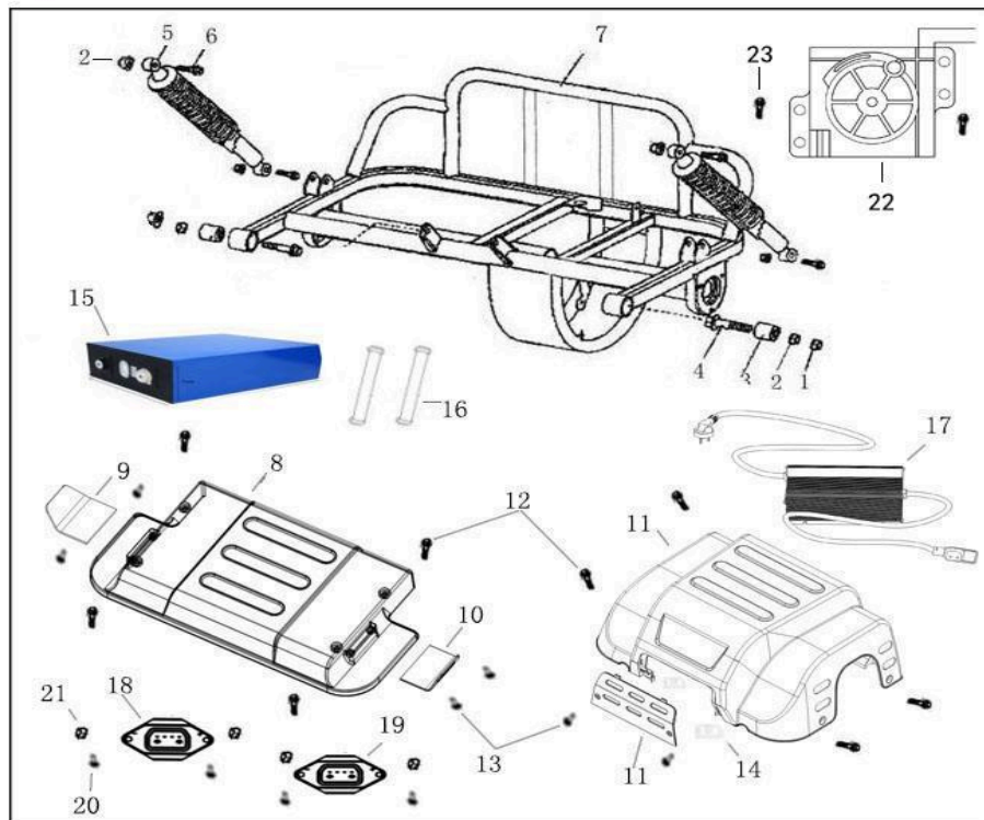
Fig 6: MOTOR/CONTROLLER ASSY
