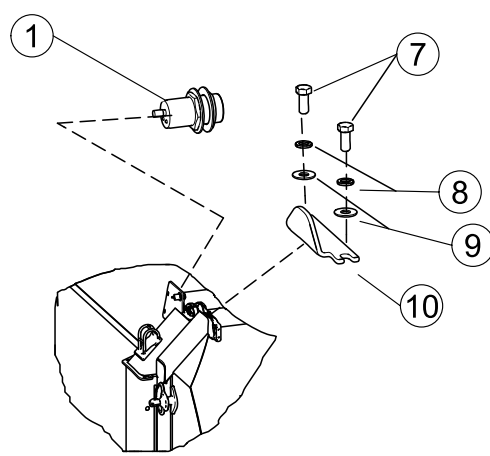
Tailgate Completely Open Sensor
