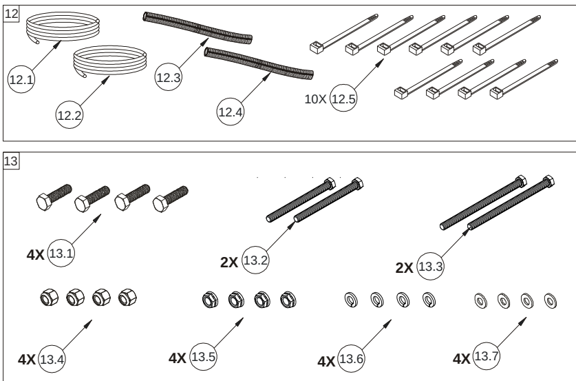
Figure 3 – Fastener Packs (cont.) (V900104)
