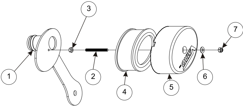
Figure 12 – Remote filter
