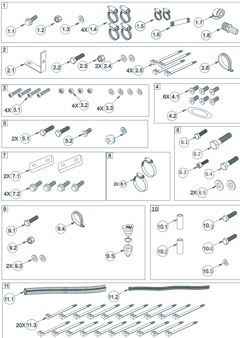
Figure 2 – Fastener Packs
