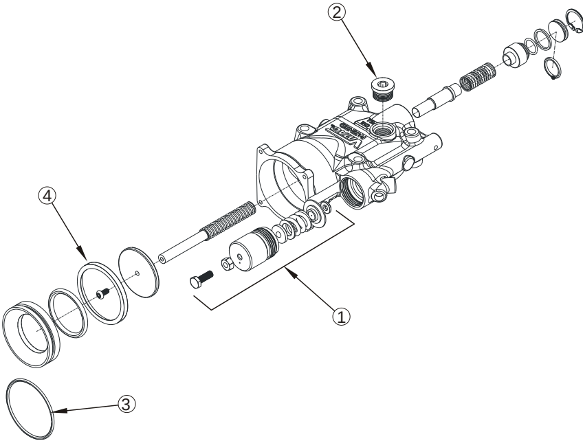
Figure 9 – Inlet Valve Sub Components
