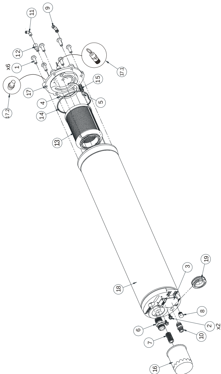
Figure 11 - VR70 Tank
