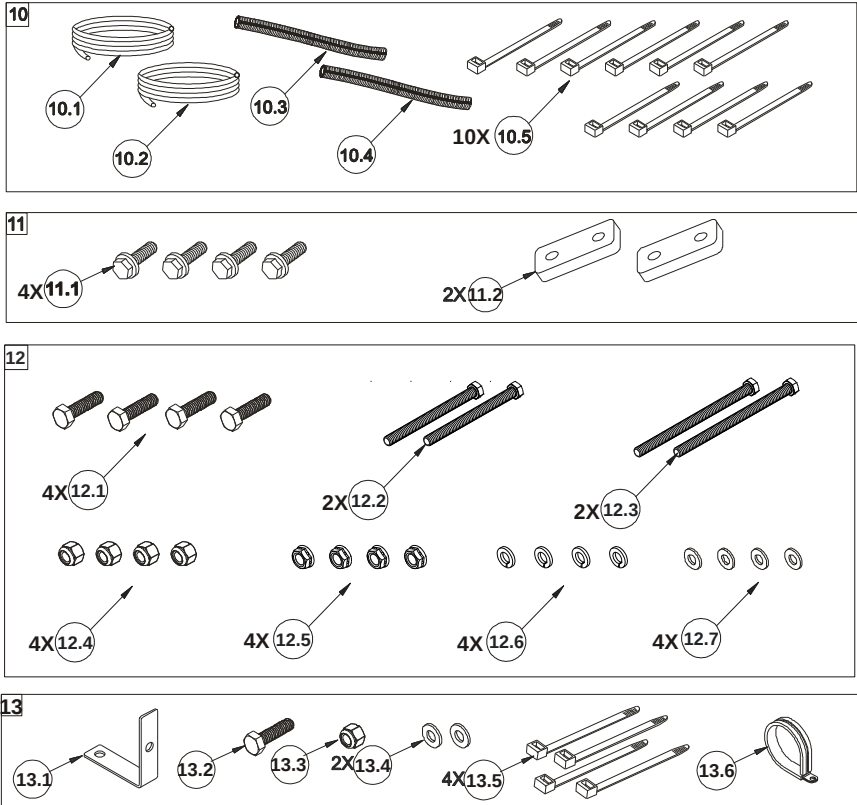
Figure 5 – Fastener Packs (cont.) (V900106)
