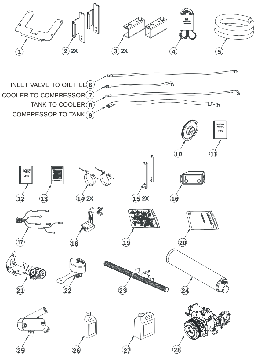
Figure 1 - Kit Pack List
