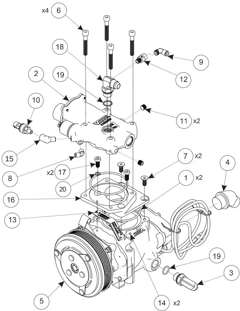
Figure 7 – Compressor Assembly (P120126)
