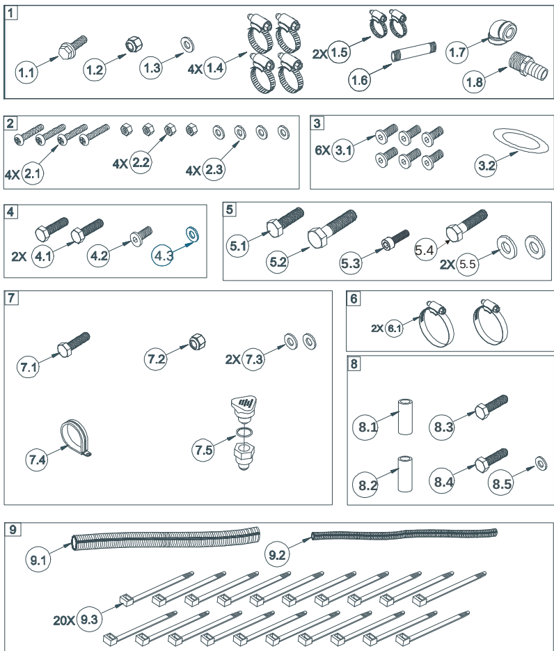
Figure 4 – Fastener Packs (V900106)
