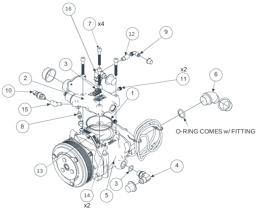
Figure 6 – Compressor Assembly (P120119)
