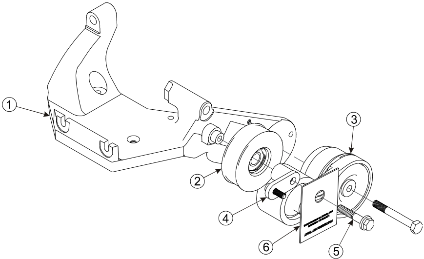
Figure 10 – Main Bracket Assembly
