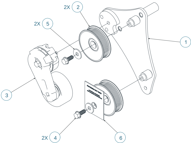
Figure 6 – Tensioner Bracket Assembly
