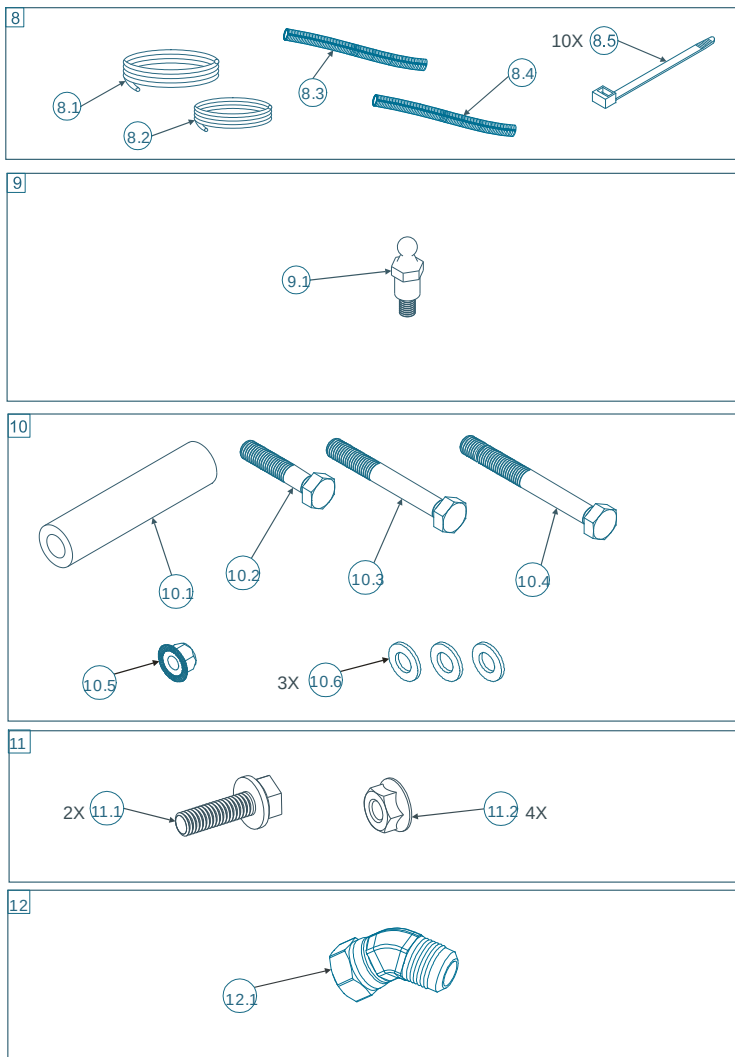
Figure 2 (Continued) – Fastener Packs
