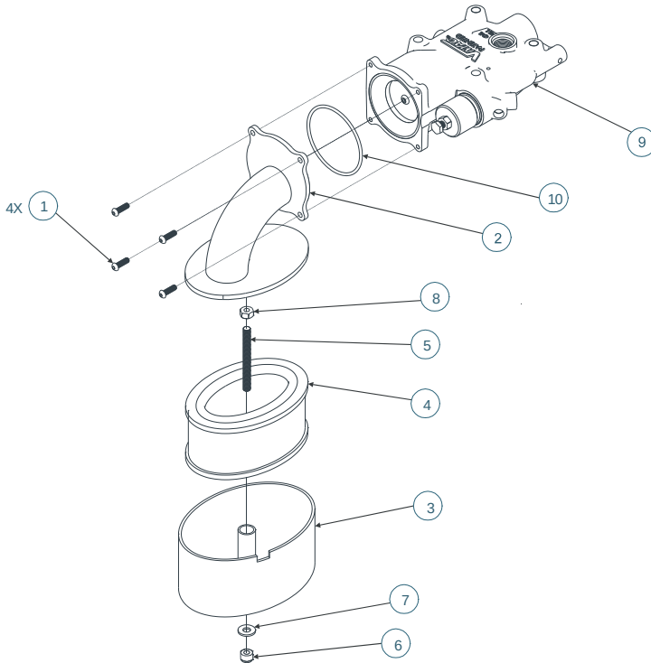
Figure 5 – Inlet Valve Sub Components
