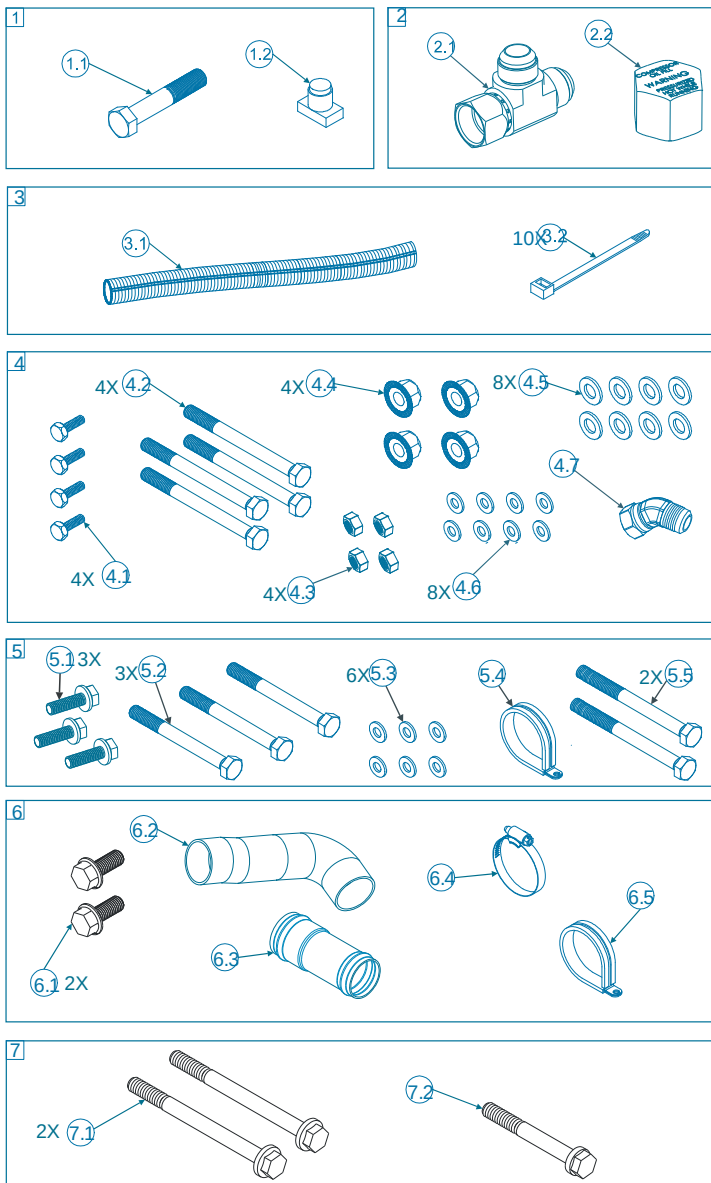
Figure 2 – Fastener Packs
