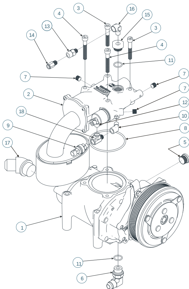
Figure 3 – Compressor Assembly
