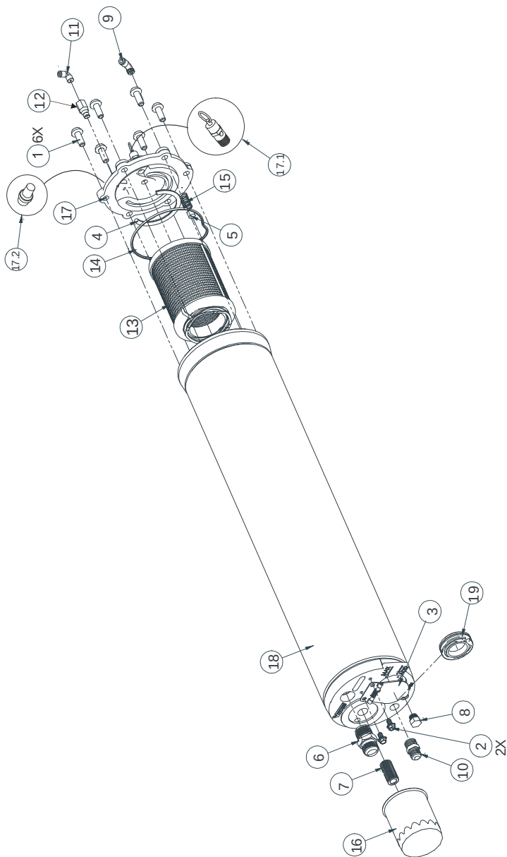
Figure 7 – Tank
