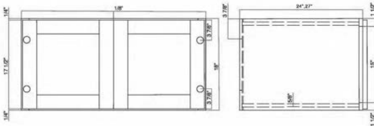
Cabinet Dimensions
