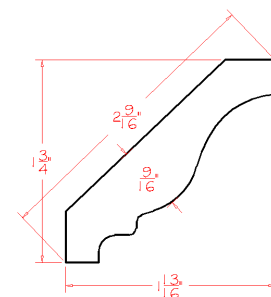
Crown Moulding - Classic Crown Moulding
