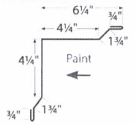
EXTENDED VALLEY BZREV
