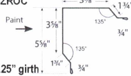
OUTSIDE CORNER BZRUC
