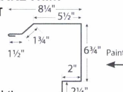
COMMERCIAL VALLEY* BZRVCV
