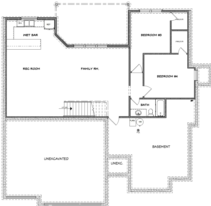
LOWER FLOOR 1371 S.F.
