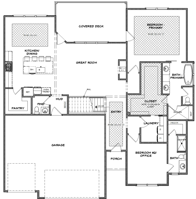
MAIN FLOOR 1918 S.F.
