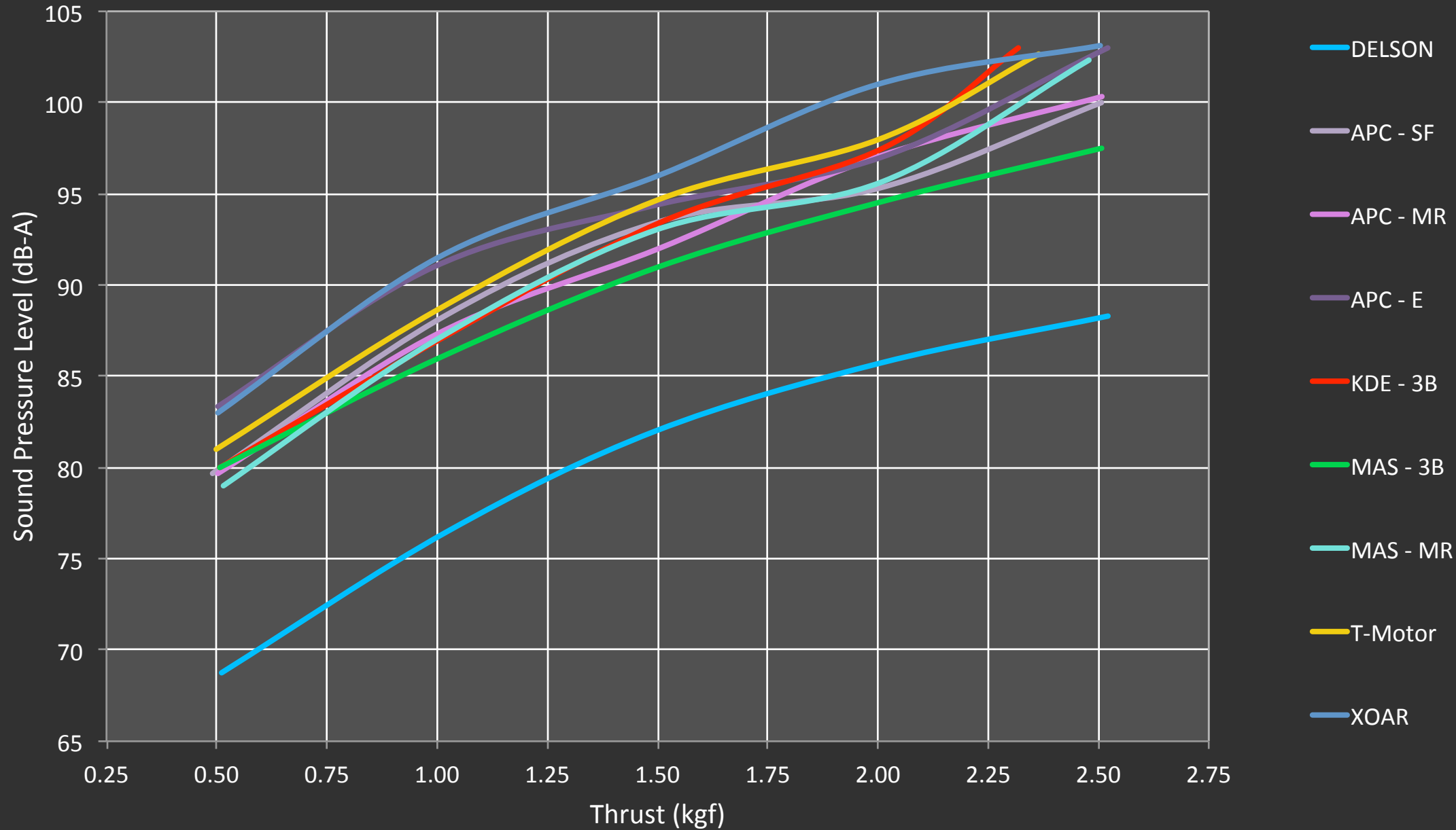
Thrust vs. Sound Pressure Level
