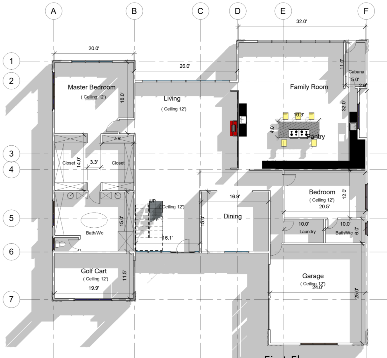
First Floor
