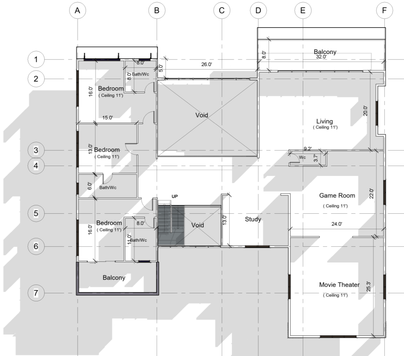
Second Floor
