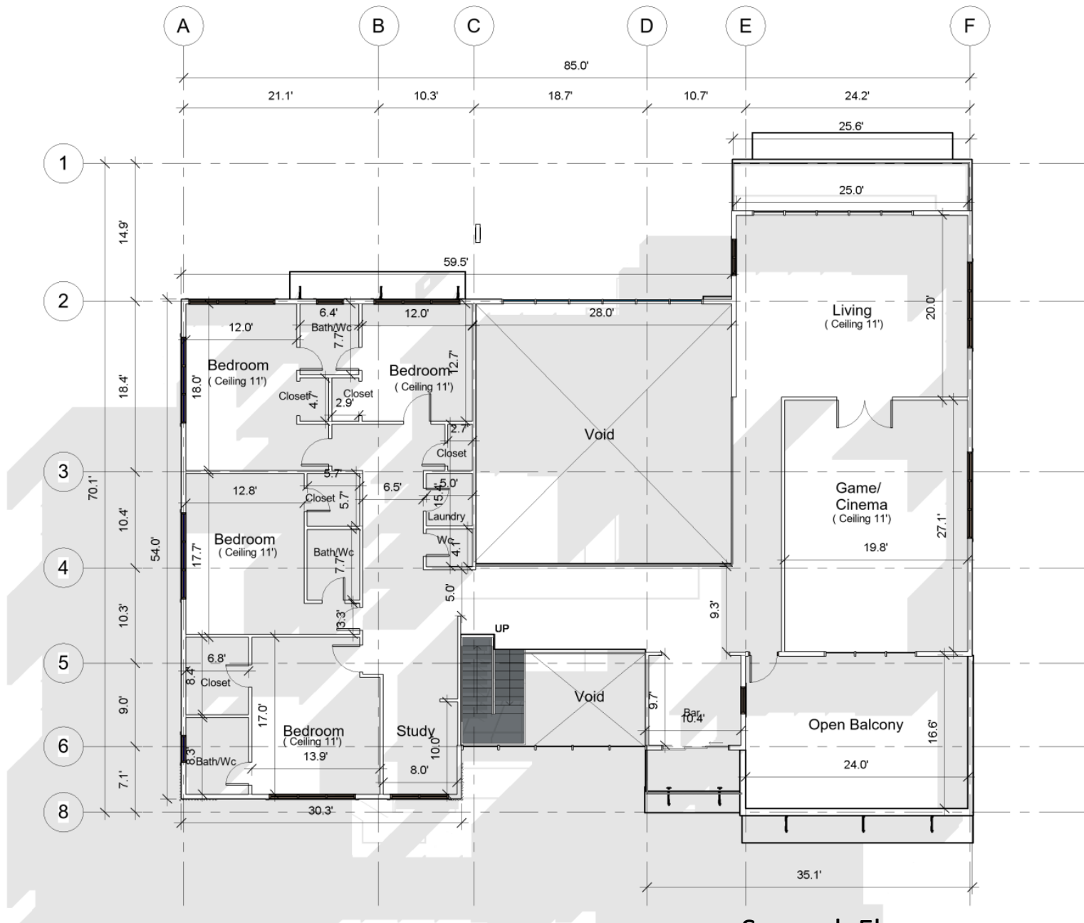
Second Floor
