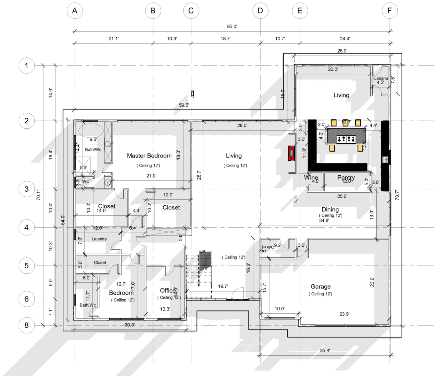
First Floor
