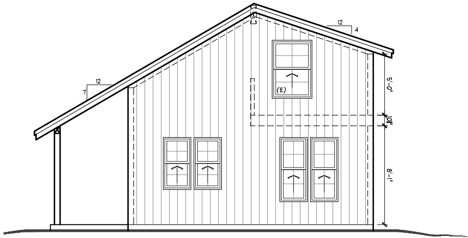
RIGHT ELEVATION 1/8" = 1'-0"
