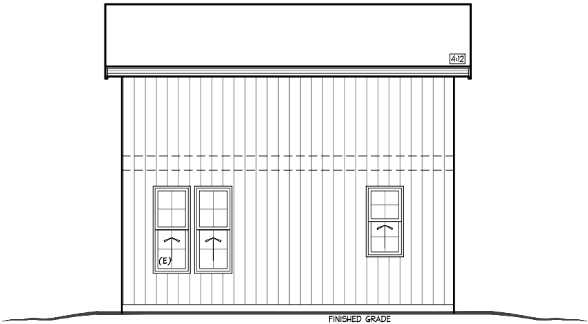
REAR ELEVATION 1/8" = 1'-0"
