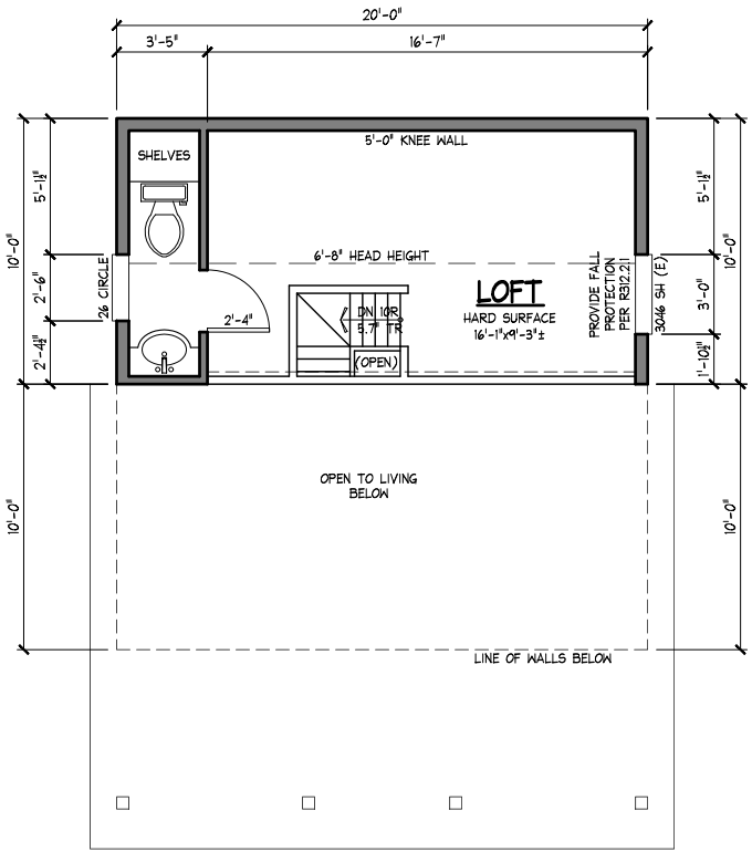
LOFT PLAN 1/8" = 1'-0"
