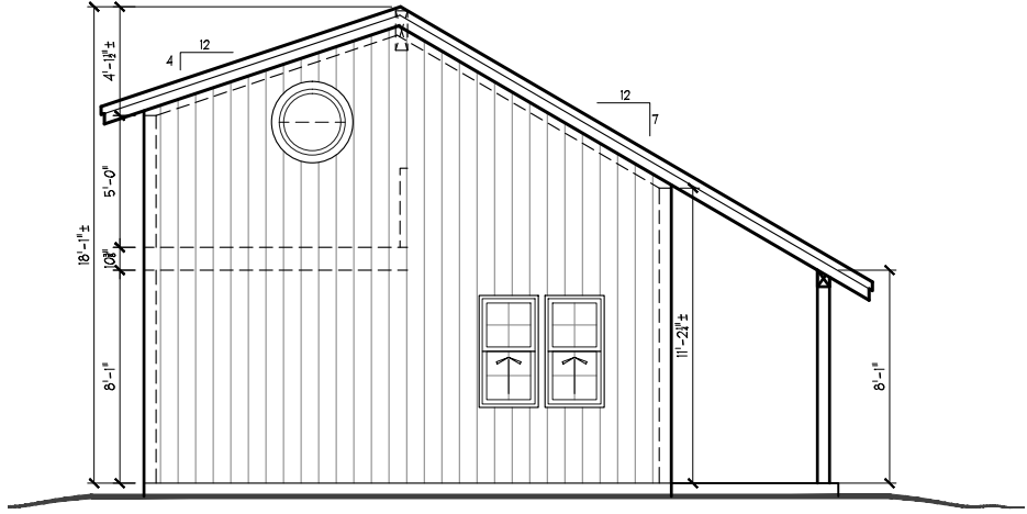
LEFT ELEVATION 1/8" = 1'-0"
