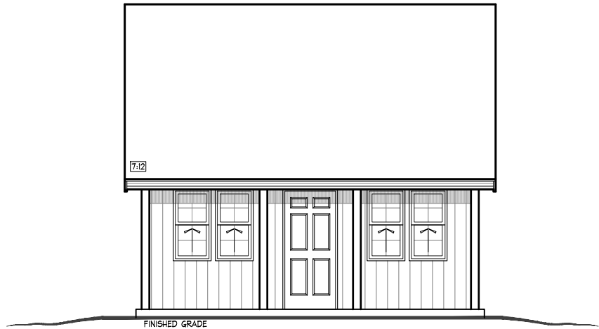
FRONT ELEVATION 1/8" = 1'-0"
