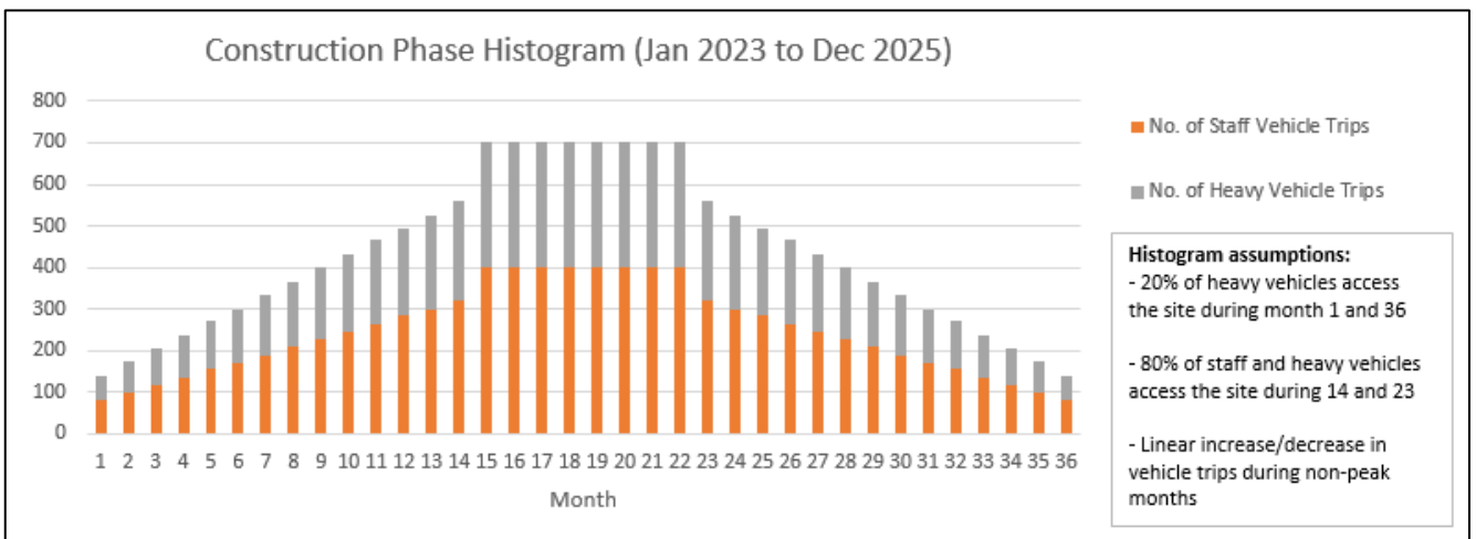
Figure 3-2: Indicative construction phase histogram – one-way daily vehicle trips
