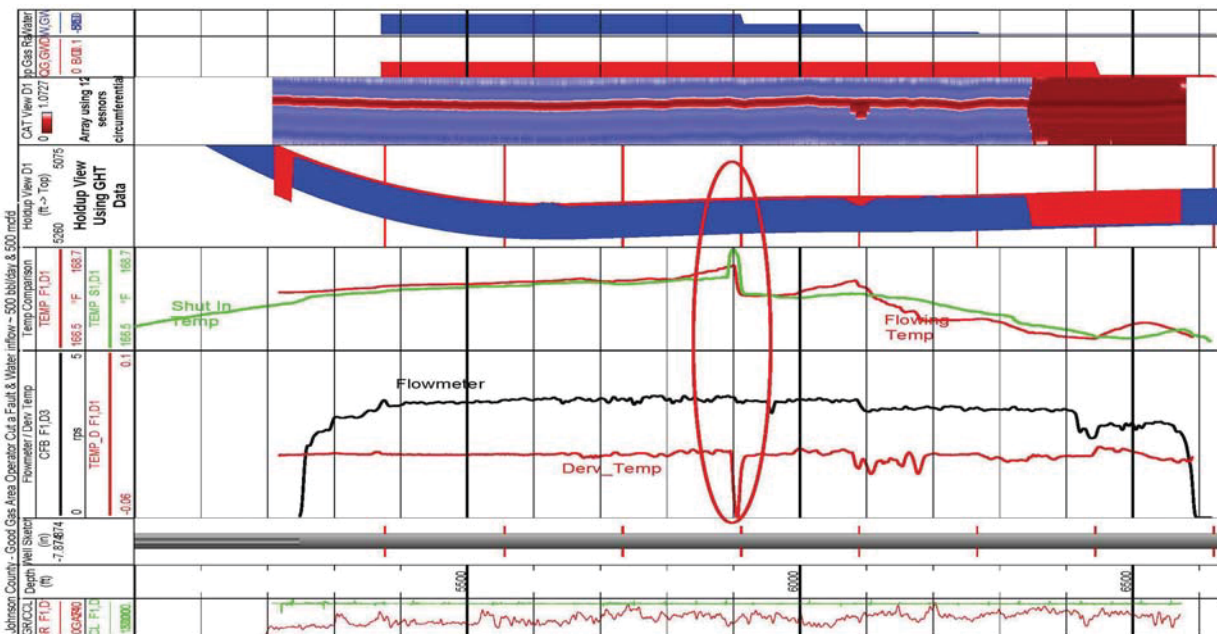
Fig 11. Array sensors compared to fullbore holdup measurements.
