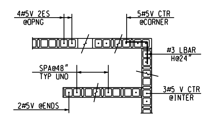
DETAIL X TYPICAL VERTICAL PLACEMENT DETAIL (DETAILS/SS.0)
