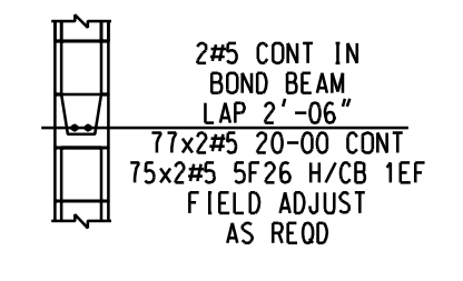
DETAIL Z (DETAILS/SS.0)
