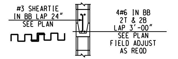
DETAIL Y (DETAILS/SS.0)
