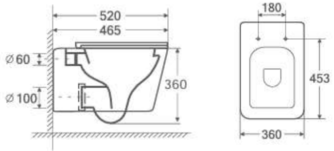
TG-WCW-111WHWH WALL HUNG WATER CLOSET
