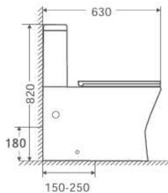
TG-WCW-662CCWH CLOSE COUPLED WATER CLOSET
