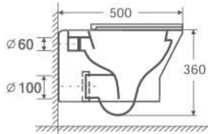
TG-WCW-662WHWH WALL HUNG WATER CLOSET
