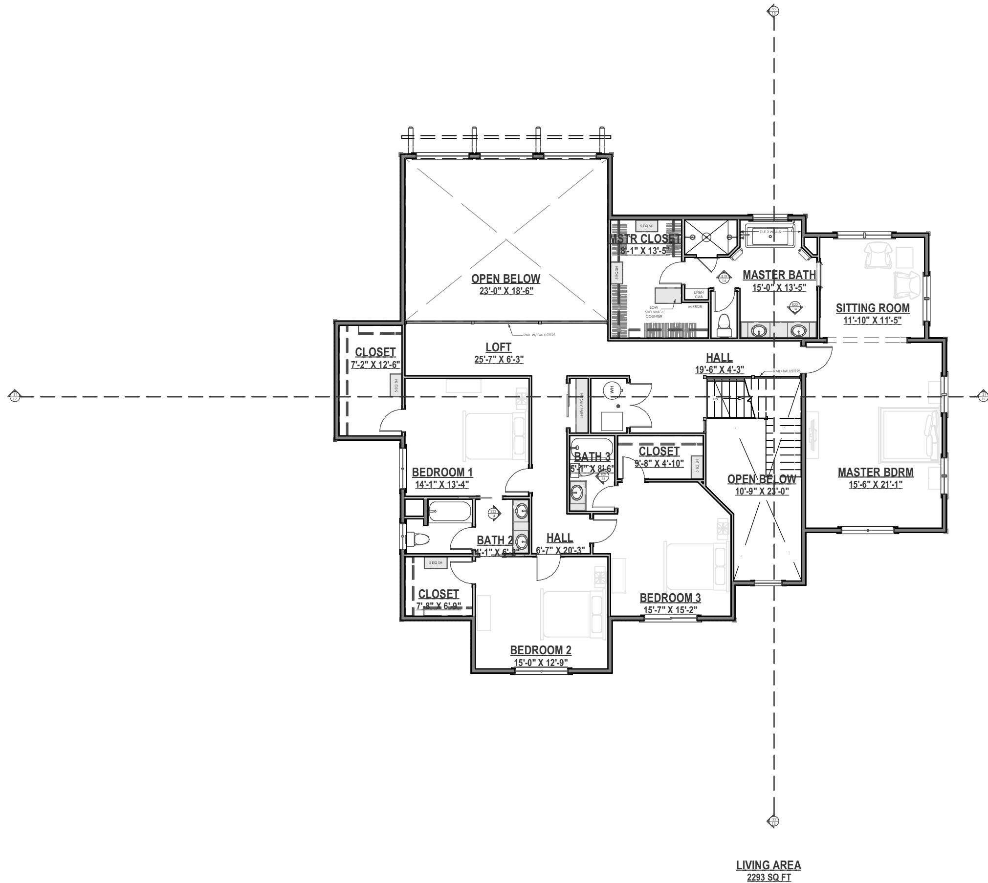
UPPER LEVEL
