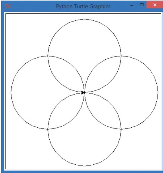
Figure 4-1: A four-circle rosette pattern
