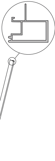
"Right Side Guide Profile"
