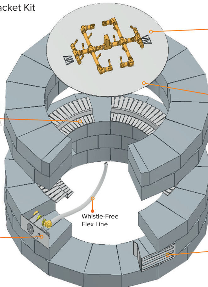
Key Valve / Mounting Bracket (Replaces one block and provides support for blocks above.)
