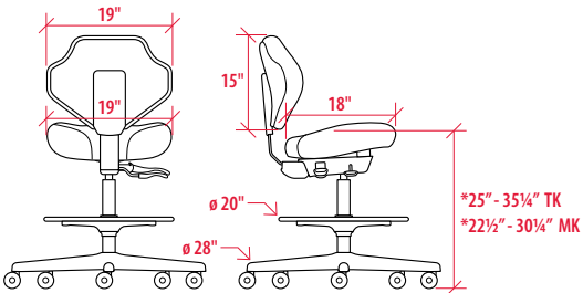
MK & TK Medium Stool Kit & Tall Stool Kit
