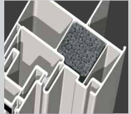
ClimaTech iE option features insulating foam inserts in select mainframe channels.
