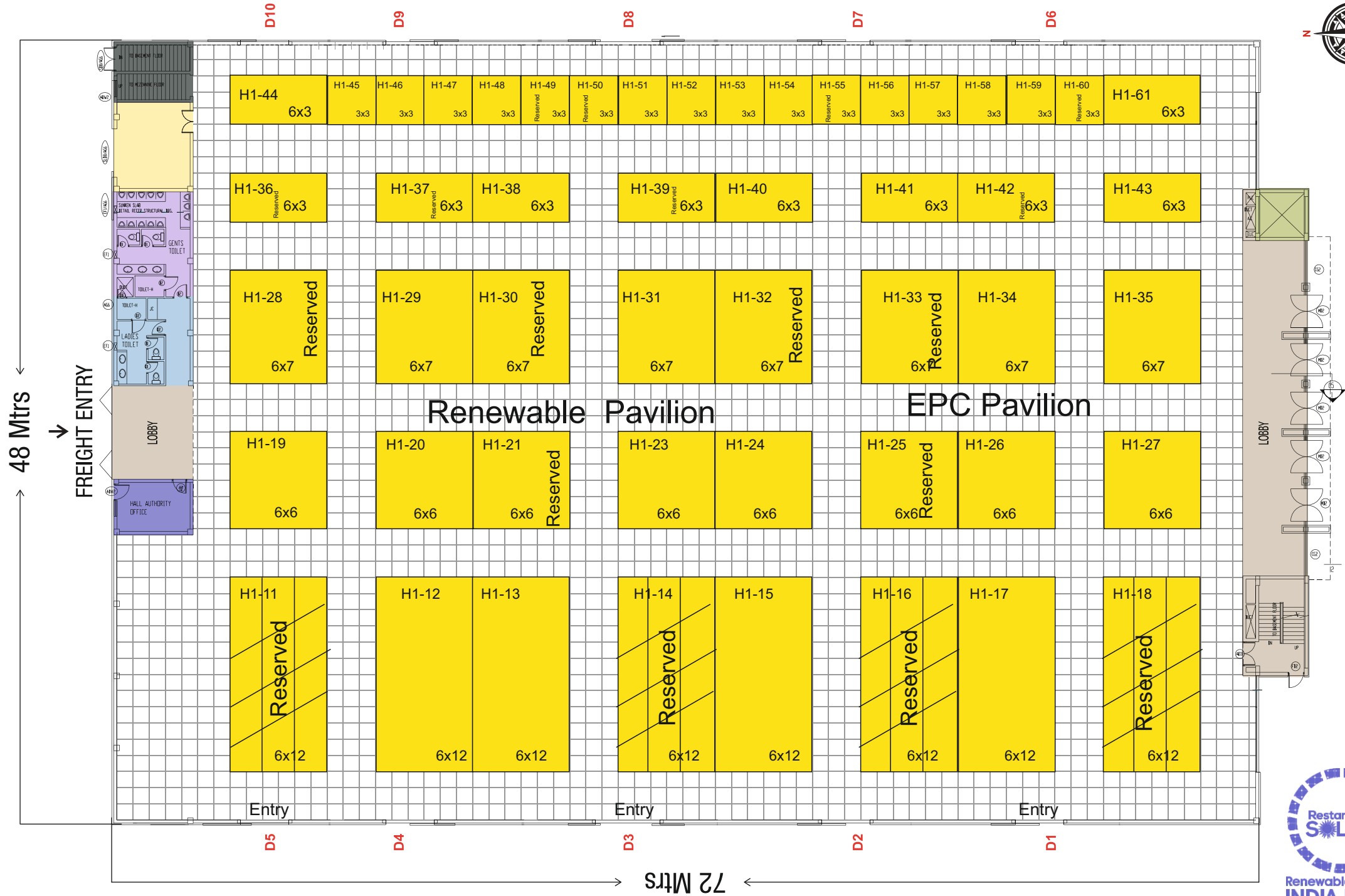
TYPICAL LAYOUT HALL 1 / 2 / 3 (3,500 Sq.M.)
