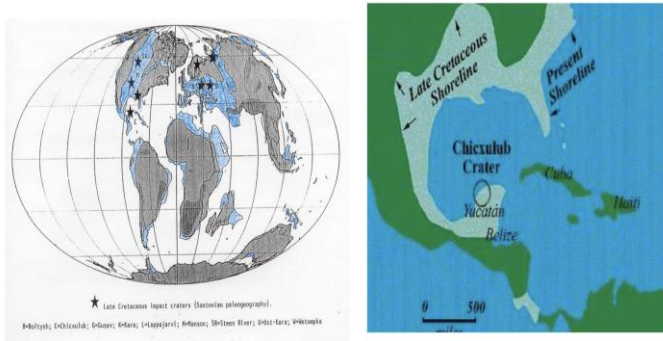
Fig. 2. Both maps here show craters formed from significant meteor impacts where these indicators could be new spots for more Primary Water Resources like the Florida location. See Right map showing the Yucatan Meteor impact creating Florida's tilted platform giving access to this Unique Primary Water Resource found by Joe Gilberti PE
