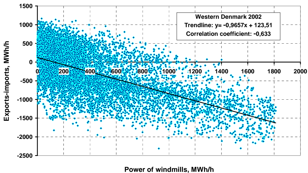
Fig. 2. Correlation between power of windmills and electricity exports-imports in Western Denmark 2002
