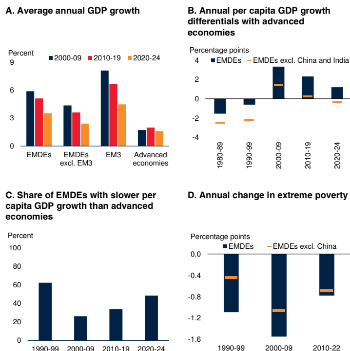
Sources: UN World Population Prospects; World Bank; World Bank Poverty and Inequality Platform. Note: EM3 = China, India, and Brazil; EMDEs = emerging market and developing economies. A. Bars show simple average for each decade of annual GDP-weighted average growth in each group of economies. Data for the 2020s include 2020-24. Growth rates for 2024 are estimated. B.C. Per capita GDP is calculated as the total GDP for each group of economies divided by the total population in each group. GDP aggregates are calculated using real U.S. dollar GDP weights at average 2010-19 prices and market exchange rates. Per capita growth rates for 2024 are estimated. D. Bars show average annual change in extreme poverty rates.
