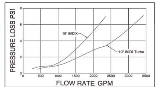
10" Model 80DI Turbo vs. 10" Model 80D1X Head Loss Comparison Chart
