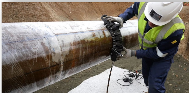
Eddy Current Array (ECA)
