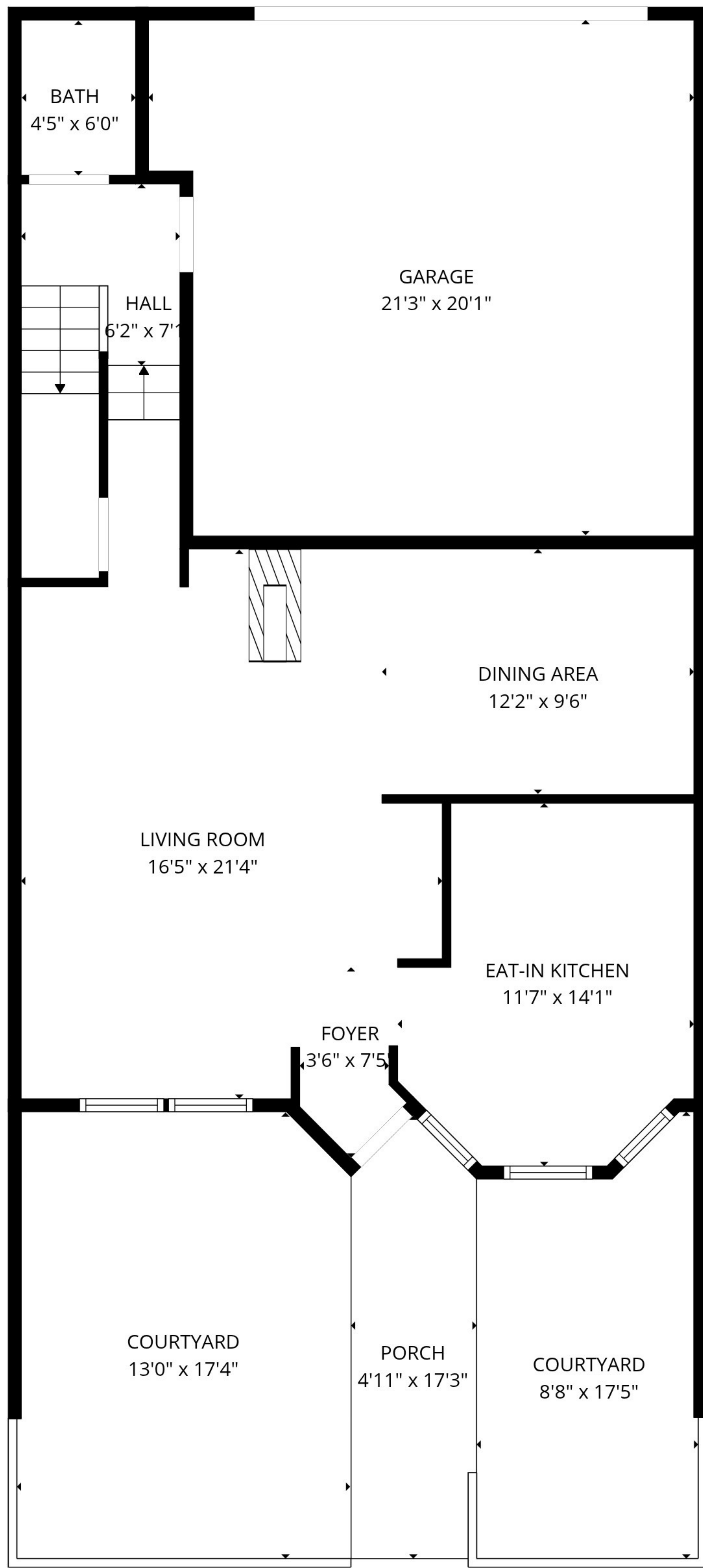
1st floor
