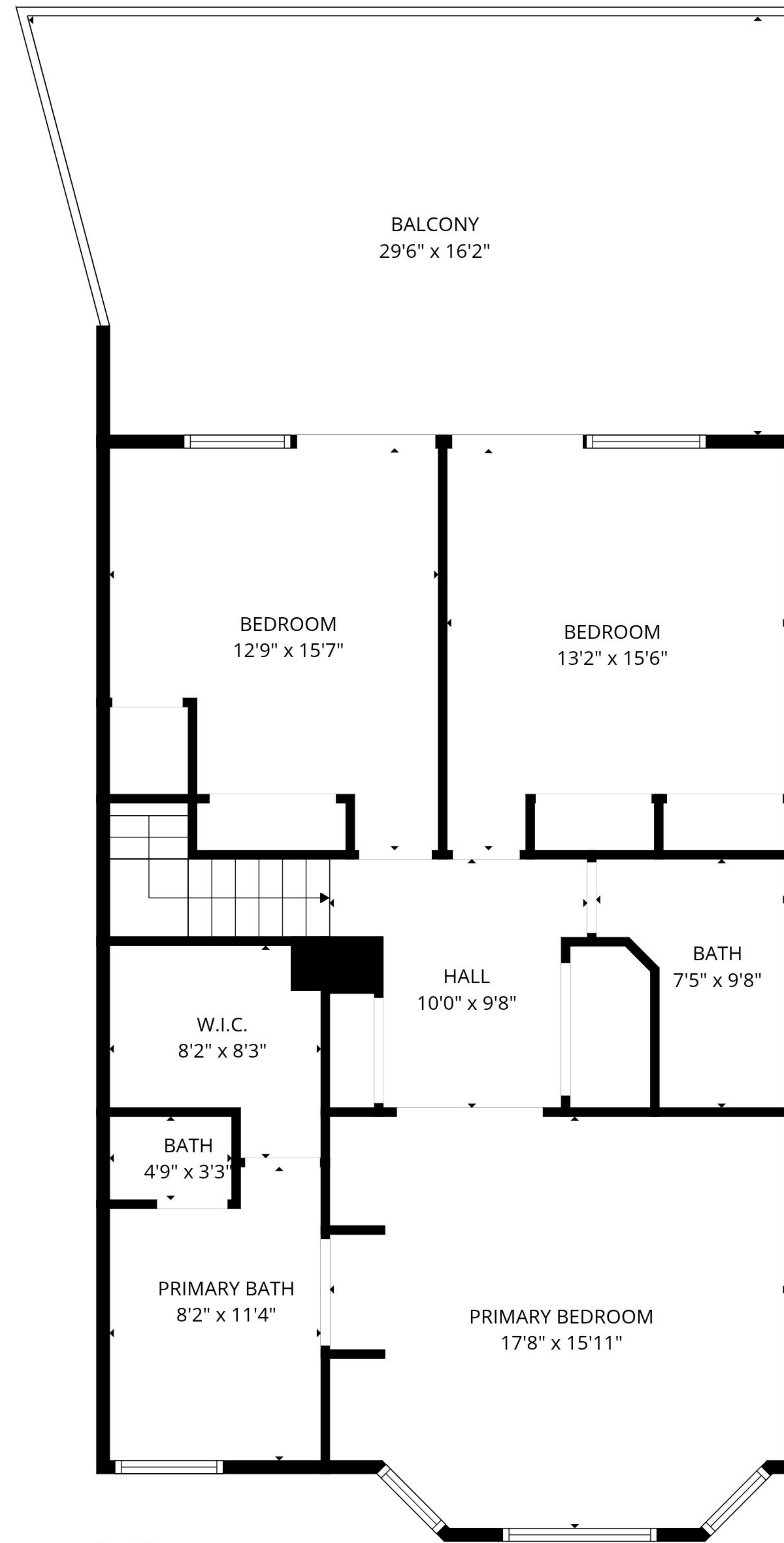
2nd floor
