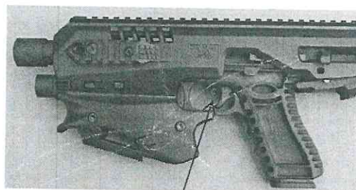
MCK with no trigger guard
