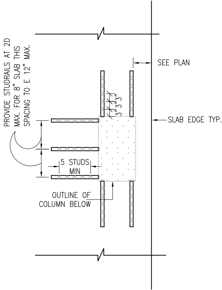
SHEAR STUDS AT EDGE COLUMN REF: S-403.00 (102017) SCALE - 1/2"=1'-0"
