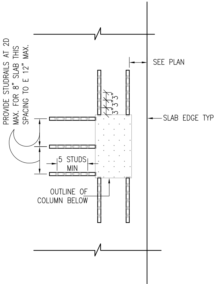
SHEAR STUDS AT EDGE COLUMN
