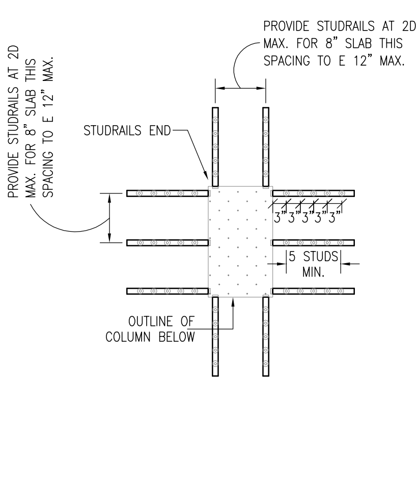
SHEAR STUDS AT INTERIOR COLUMN REF: S-403.00 (102017) SCALE - 1/2"=1'-0"
