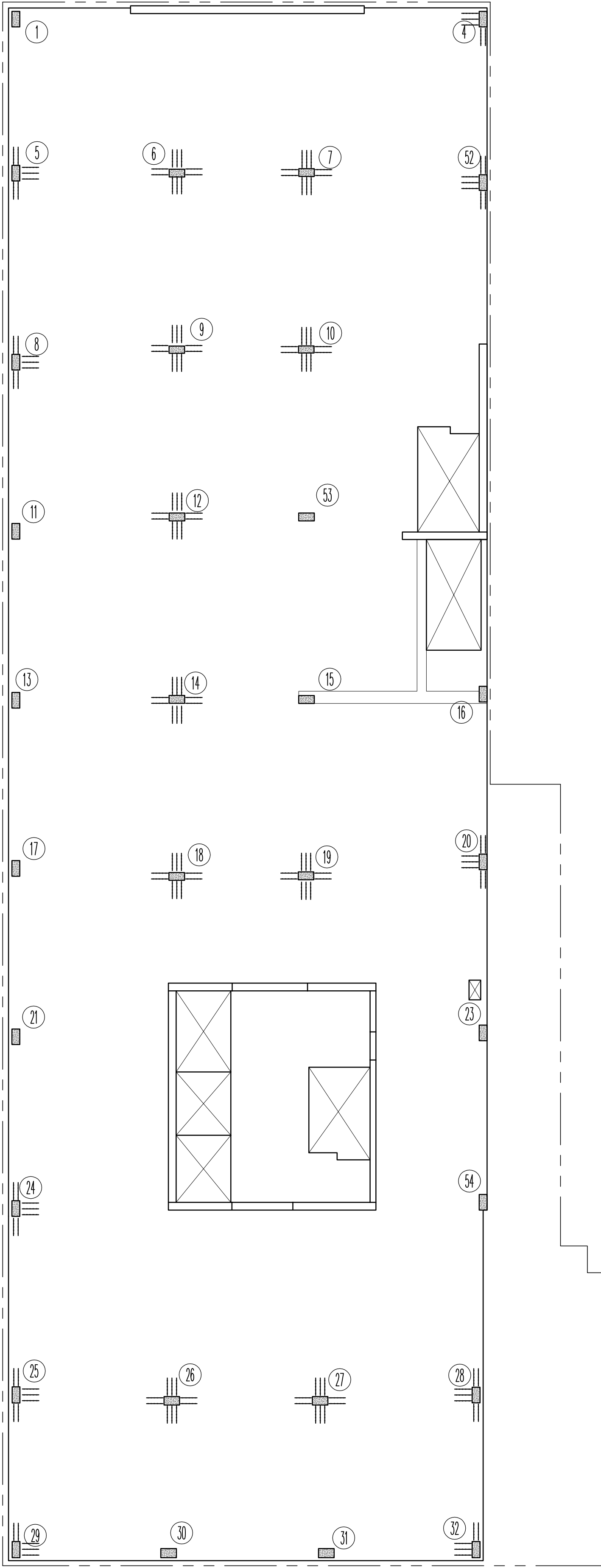
THIRD TO FIFTH FLOOR- COLUMN REFERENCE PLAN REF: S-103.02 (102017) SCALE - 3/32"=1'-0"
