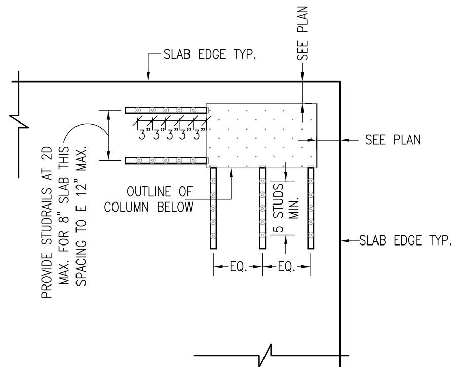
SHEAR STUDS AT CORNER COLUMN REF: S-403.00 (102017) SCALE - 1/2"=1'-0"
