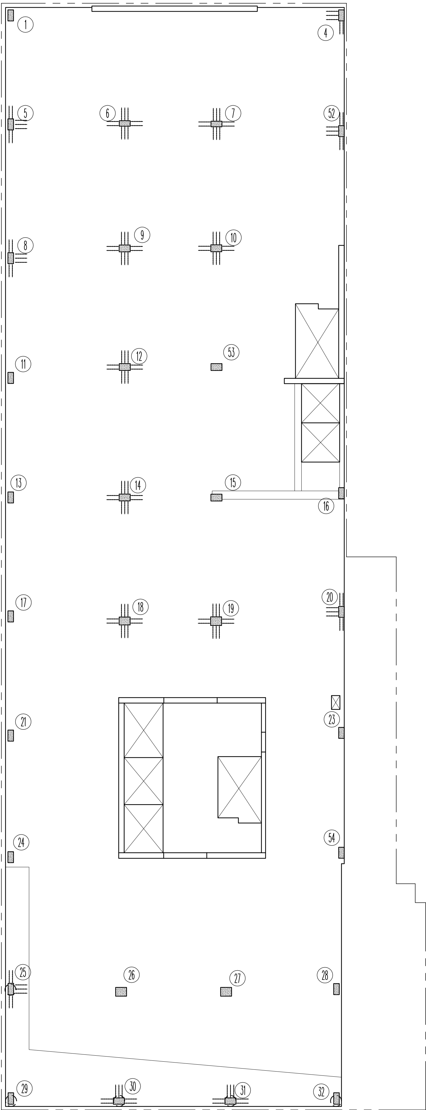
SECOND FLOOR— COLUMN REFERENCE PLAN REF: S-101.02 (102017) SCALE - 3/32"=1'-0"
