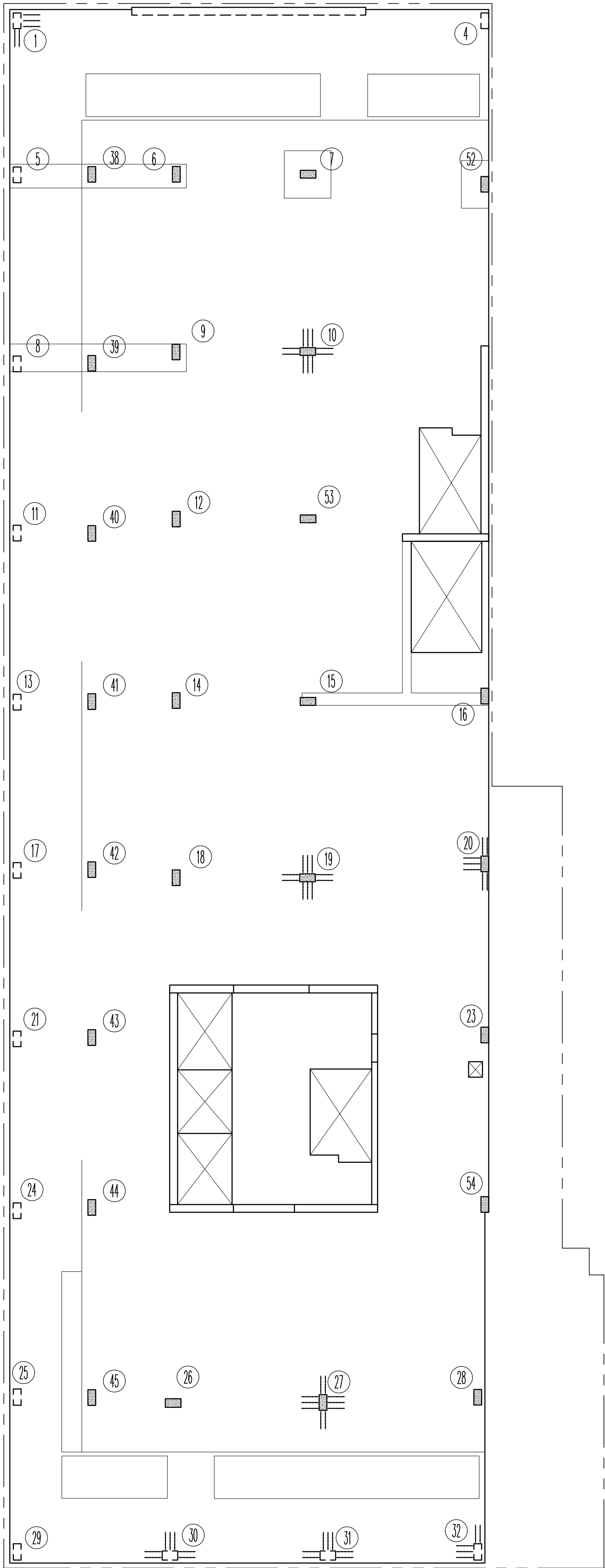
SIXTH FLOOR- COLUMN REFERENCE PLAN REF: S-103.02 (102017) SCALE - 3/32"=1'-0"
