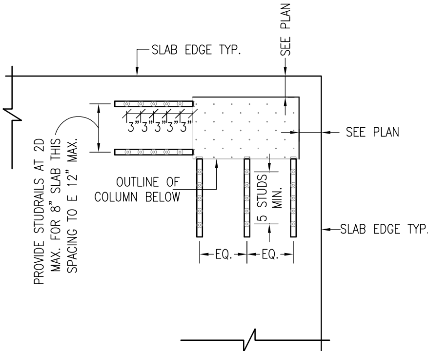
SHEAR STUDS AT CORNER COLUMN
