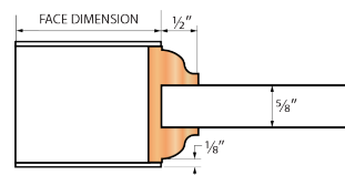
Flat Panel
