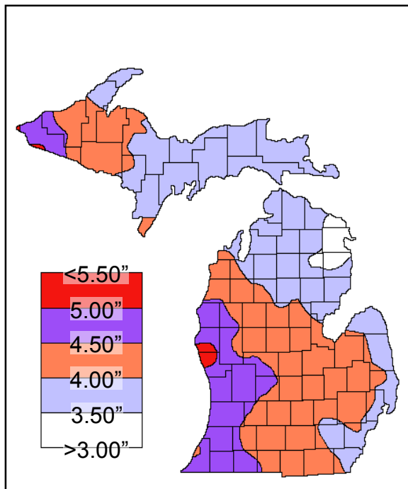
Figure 6. 4% Annual Exceedance Probability, 24-Hour Precipitation Source: NOAA, 2013.
