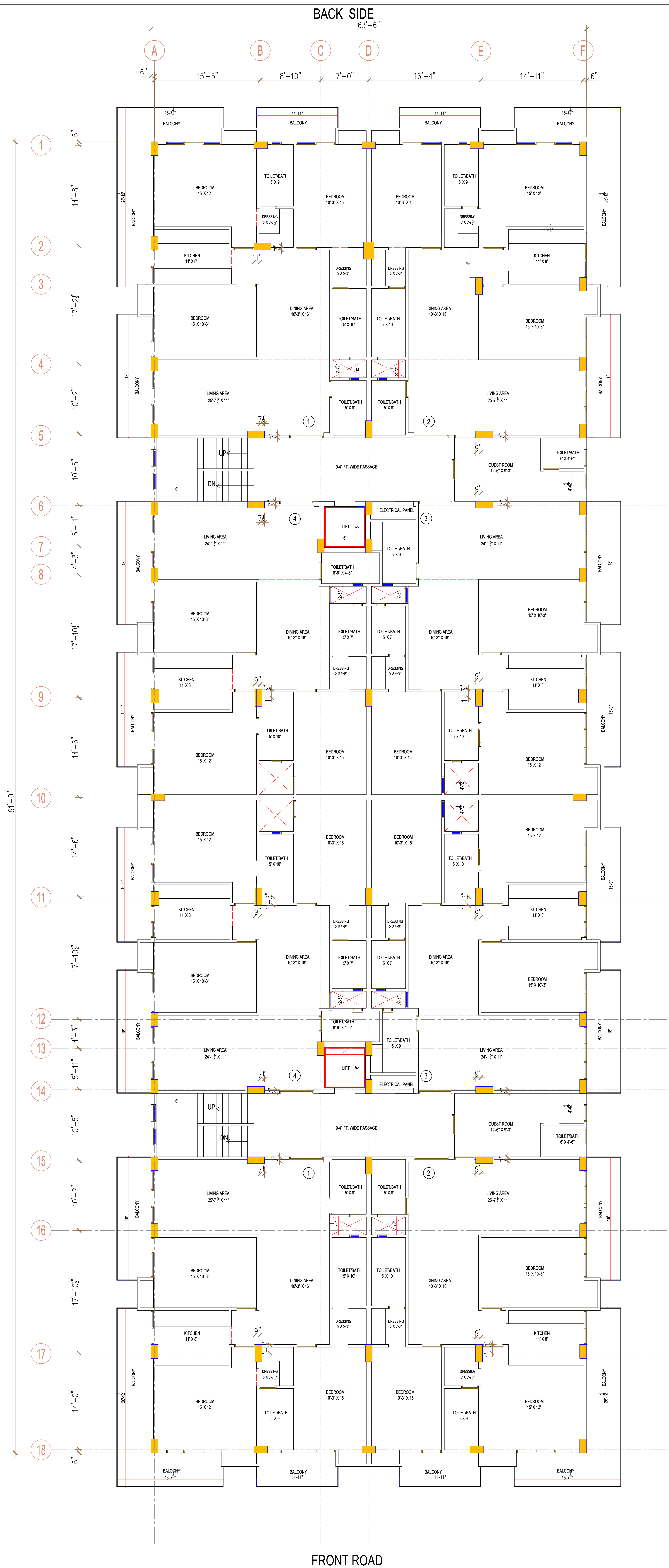
TYPICAL FLOOR PLAN
